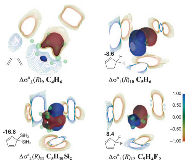
Figure 4. Isosurface plots (1 ppm value) of the out-of-plane shielding tensor component difference: \Delta\sigma^\pi_\perp(R) for 9–12 at the same levels as given in Figure 3. Standard NICS(0) _{\pi_{zz}} values are in bold. Note the similarities between \Delta\sigma^\pi_\perp(R)_{11} and \Delta\sigma^\pi_\perp(R)_1 for benzene as well as between \Delta\sigma^\pi_\perp(R)_{12} and \Delta\sigma^\pi_\perp(R)_4 for cyclobutadiene. See the Supporting Information for details.
