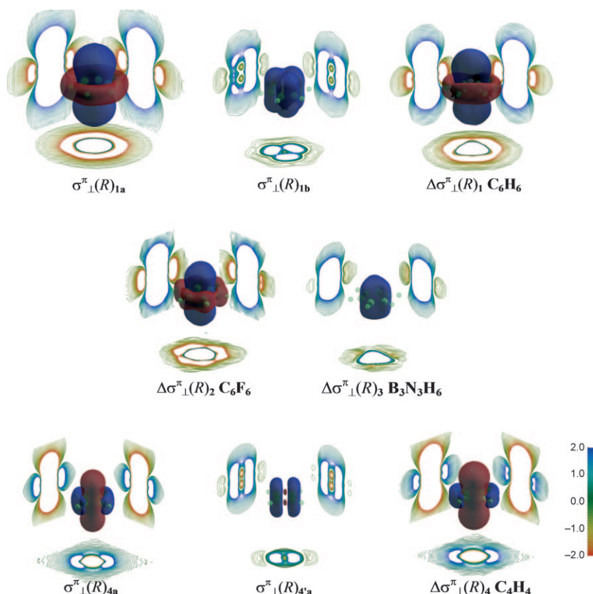
Figure 3. Isosurface plots (2 ppm value) of the out-of-plane shielding tensor components, and the shielding differences \Delta\sigma_{\perp}(R) between the fully delocalized (e.g. \sigma_{\perp}^{\pi}(R)_{1a} for 1a , D_{6h} ) and block-localized (e.g. \sigma_{\perp}^{\pi}(R)_{1b} for 1b , D_{6h} ) structures of benzene ( 1 ), hexafluorobenzene ( 2 ), borazine ( 3 ), and cyclobutadiene ( 4 ). Shielding/deshielding zones are indicated in blue/red. Magnetic shielding computations at (BLW)-IGLO-PW91/IGLO-III employed standard (i.e. non-BLW) B3LYP-6-31G* geometries. The hydrogen and heavy atoms locations are indicated by small and large light green spheres, respectively.
