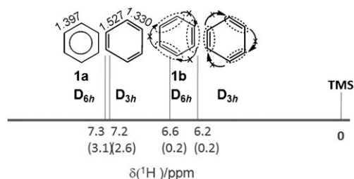
Figure 1. (BLW)-IGLO-PW91/IGLO-III isotropic NMR \delta(^1\text{H}) chemical shifts for 1a and 1b (the \pi contribution to the out-of-plane shielding tensor components \delta^\pi_\perp are given in parentheses) referenced to the experimental benzene proton chemical shift ( \delta = 7.27 ). [1] Geometries were optimized at B3LYP/6-31G(d) for D_{6h} 1a and 1b and at BLW-B3LYP/6-31G(d) (fully optimized with the BLW constraints) for D_{3h} 1a and 1b . Bond lengths are in Å. Blocked double bonds are circled.
