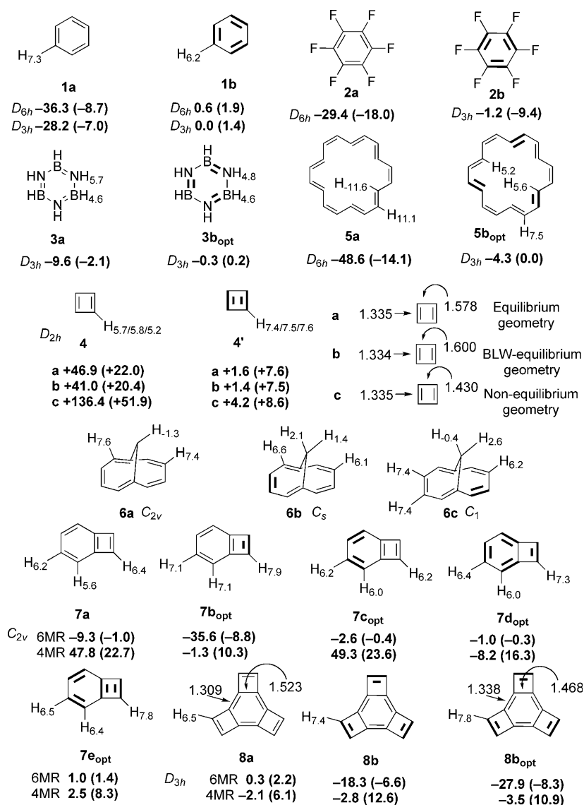
Figure 2. (BLW)-IGLO-PW91/IGLO-III isotropic NMR δ( 1 H) chemical shifts referenced to the experimental benzene proton chemical shift (δ = 7.27 ppm) [1] employing B3LYP/6-31G(d) geometries (BLW indicated as opt ). Blocked double bonds are indicated in bold. NICS(0) πzz /NICS(0) isotropic values were computed at the individual ring centers. Owing to the nonplanarity of the π system, the 6b geometry was not optimized with BLW. More details are given in the Supporting Information.
